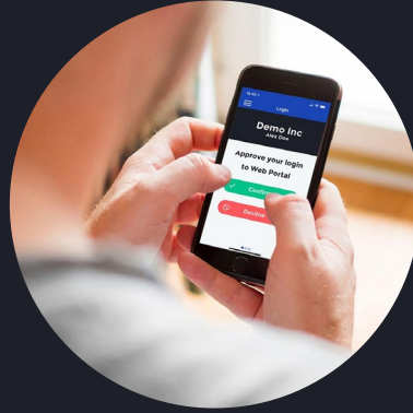
User Authentication
