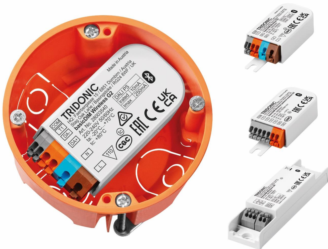
Tridonic basic DIM Wireless G2 modules
